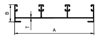
3 TRACK TOP
