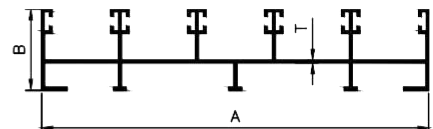
5 TRACK TOP
