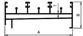
3 TRACK BOTTOM
