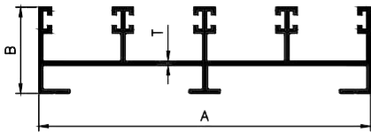
4 TRACK TOP
