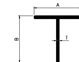
EQUAL "T" SECTION
