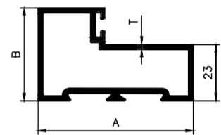
LEG SINGLE PARTITION
